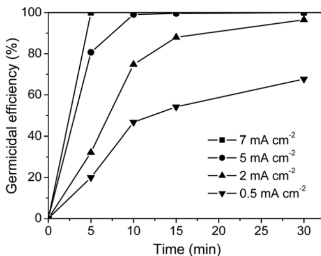
Fig. 1. Bacteria killing efficiency of electrochemical disinfection by radical intermediates. Operation conditions: Coliforms density 8.56 \times 10^5 cfu \text{mL}^{-1} ; \text{Na}_2\text{SO}_4 5 g \text{L}^{-1} ; T 25^\circ\text{C} ; pH 6.78; volume 500 mL.
